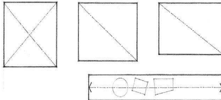
Figure 2: shapes with different ratio
