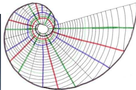
Figure (14): shows the golden spiral city plan
